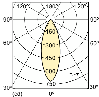
Light Distribution Diagram - CorePro LEDspotMV 5-50W GU10 827 36D RS
