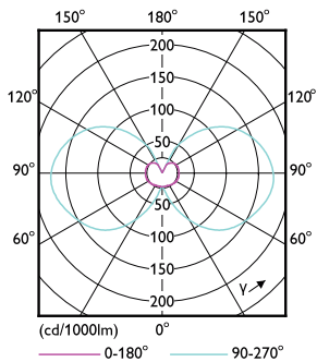
LEDcapsule CorePro 1.7-20W GY6.35 Capsule 827 ND
