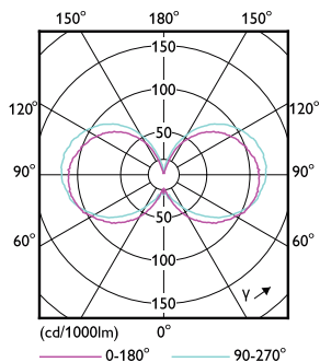
Light Distribution Diagram - CLA LEDLuster D 4.5-40W P45 E14 827 CL
