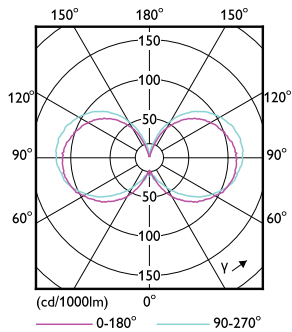
Light Distribution Diagram - CLA LEDBulb D 4.5-40W A60 E27 827 CL
