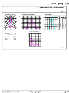
MAS LEDspotLV 43W GU5-3 927 36D MR16
