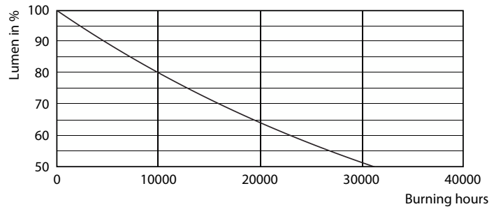
Lumen Maintenance Diagram - CLA LEDLuster ND 4.3-40W E27 827 P45 FR
