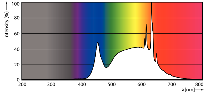
Spectral Power Distribution Colour - MAS LEDspotLV D 20-100W 940 AR111 45D
