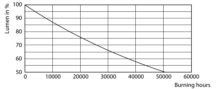
Lumen Maintenance Diagram - MAS LEDspotLV D 20-100W 940 AR111 45D
