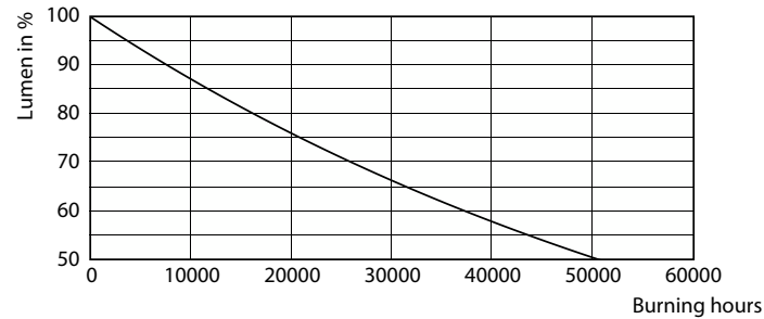
Lumen Maintenance Diagram - MAS LEDspotLV D 20-100W 927 AR111 45D
