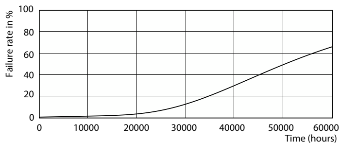
Life Expectancy Diagram - MAS LEDtube 1500mm HO 20W830 T8
