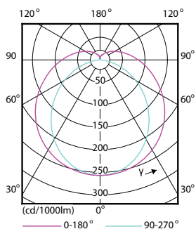
Light Distribution Diagram - MAS LEDtube 1500mm HO 20W830 T8
