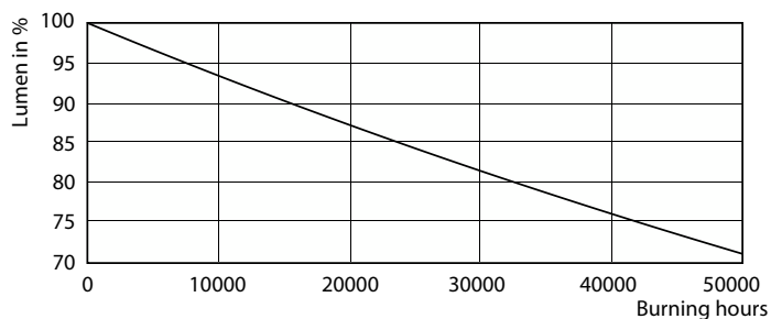
Lumen Maintenance Diagram - MAS LEDtube 1500mm HO 20W830 T8
