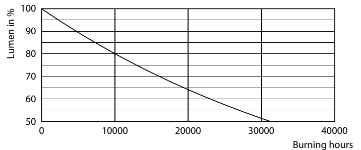
Lumen Maintenance Diagram - CLA LEDLuster DT3.5-25W E27 CRI90 P45 CL
