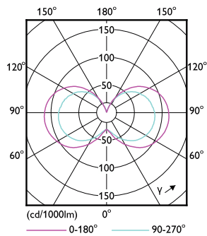
Light Distribution Diagram - CLA LEDLuster DT3.5-25W E27 CRI90 P45 CL
