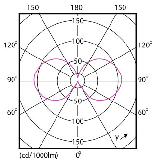
Light Distribution Diagram - CLA LEDCandle ND 4-40W B35 E14 827 CL
