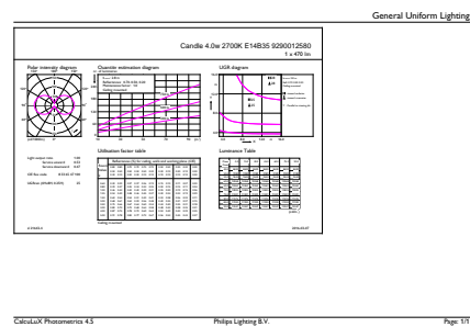
General uniform lighting - CLA LEDCandle ND 4-40W B35 E14 827 CL
