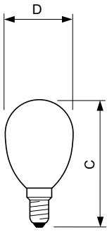
Fila P45 230V 5W-40W 470lm 2700K E14 ND
