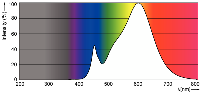
Spectral Power Distribution Colour - CorePro LEDbulb 6-40W 830 E27
