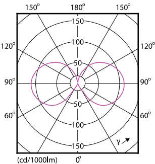
Classic LEDCandle ND 2-25W BA35 827 CL
