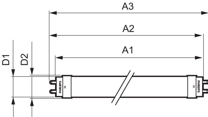
MASTER LEDtube GA110 600mm 10W 840 C
