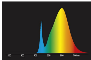
LED retrofit standard lamps 25W replacement, 2700K
