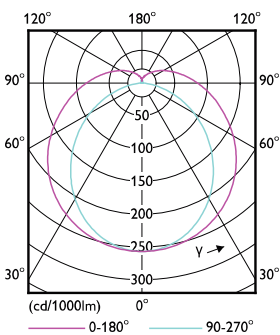
TLED_4ft_220-240V15.5-36W_G13-LDD
